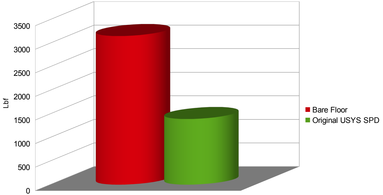
Tibia Force Lft High load case 85mm Travel in 6ms
